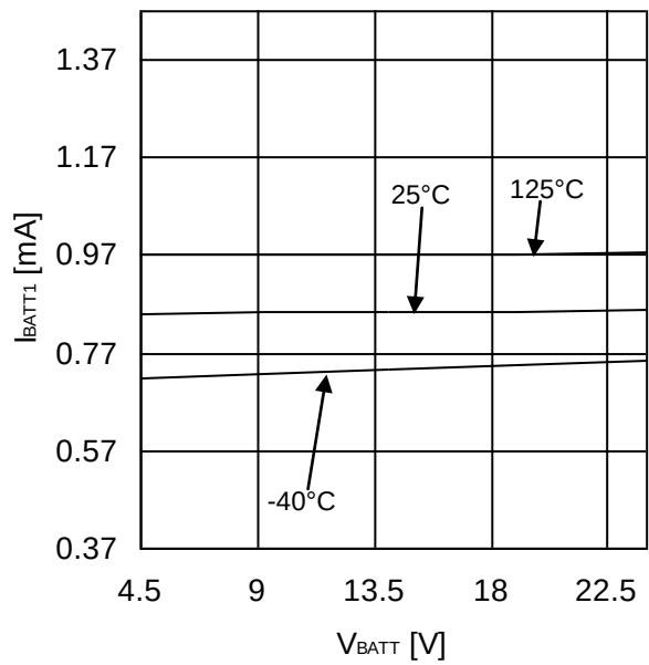
Figure 3. Main Power Supply Circuit Current 1 (FET_G Pin switching operating)
