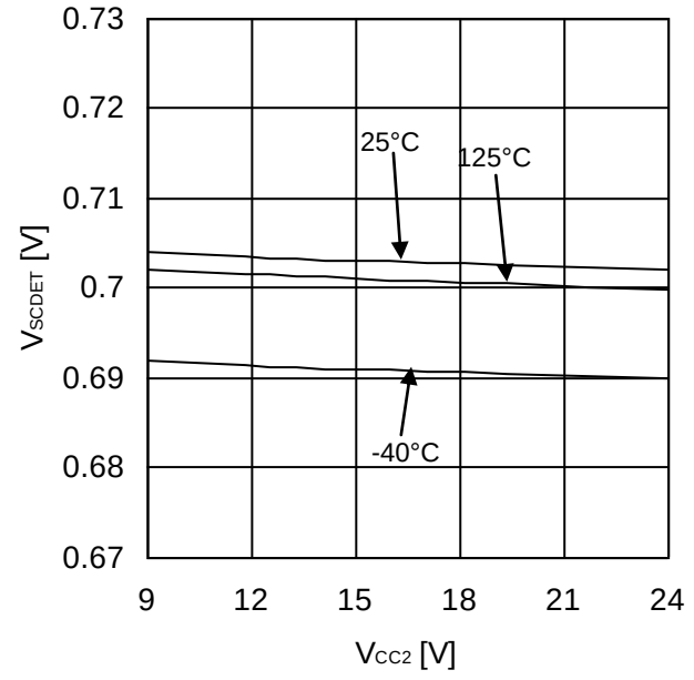
Figure 66. Short Current Detection Voltage
