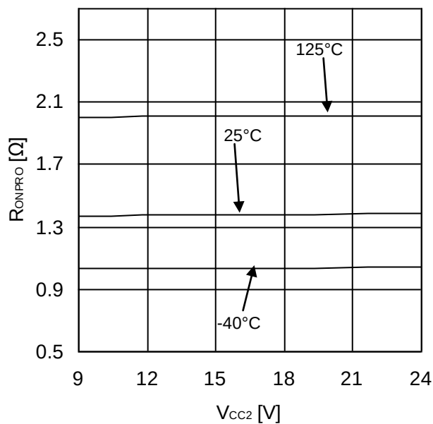
Figure 43. PROOUT ON-Resistance (I PROOUT =40mA)
