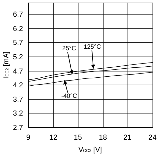
Figure 15. Output Side Circuit Current (OUT=L, R_{TC}=10k\Omega )
