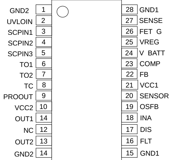
Figure 2. Pin configuration
