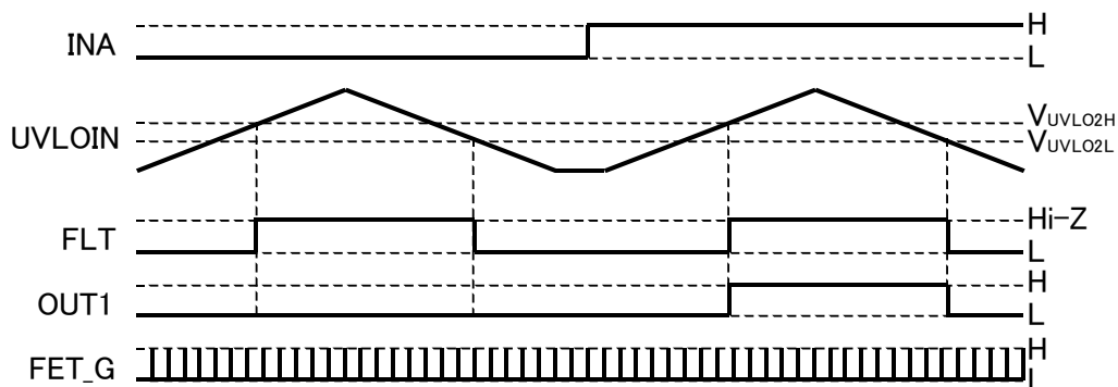
Figure 81. VCC2 UVLO Function Operation Timing Chart
