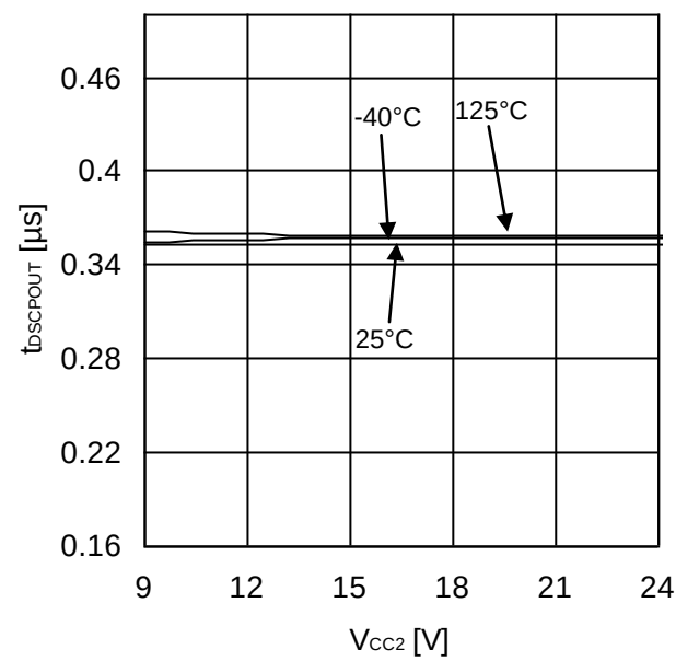
Figure 68. Short Current Detection Delay time (OUT1)
