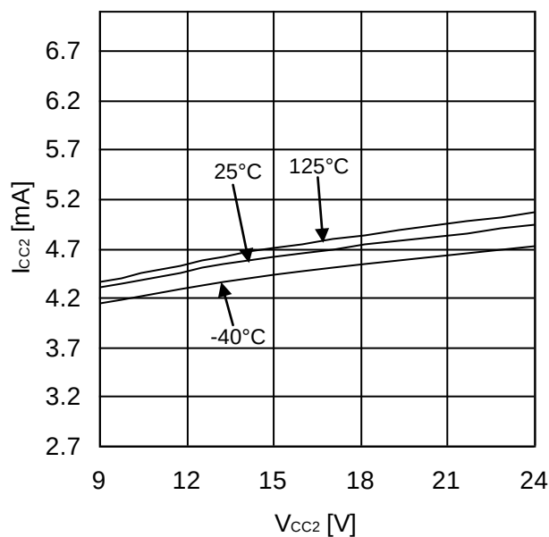
Figure 17. Output Side Circuit Current (OUT=H, R_{TC}=10k\Omega )
